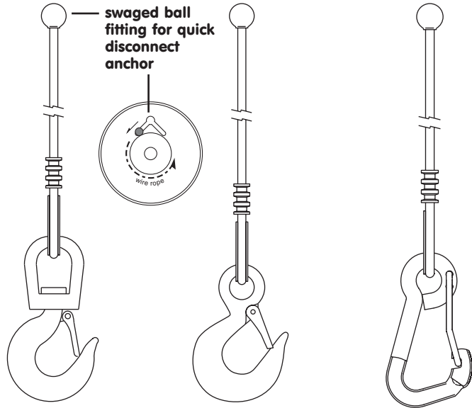
Swivel Hook
